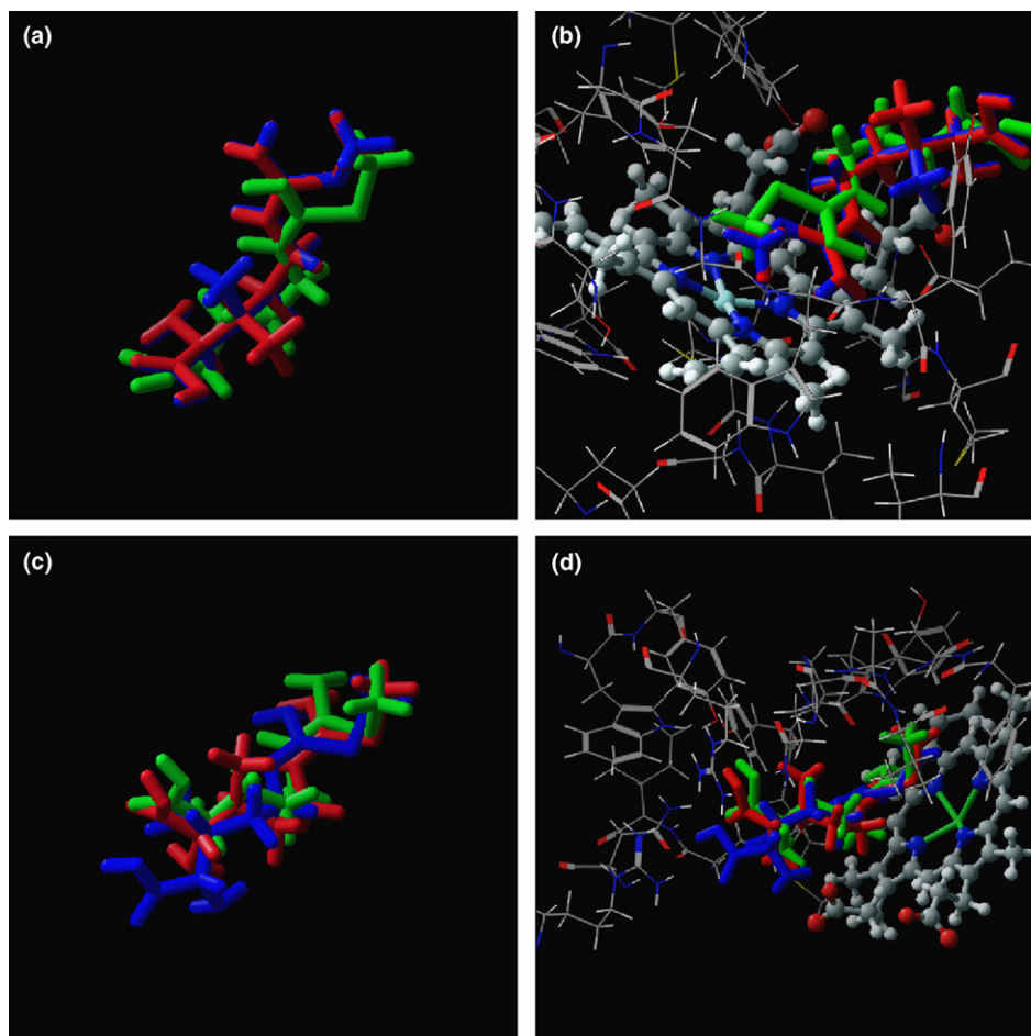
Figure 3. Superposition of the minimum energy conformations of 1 (green) and 4 (blue) and 5 (red) in the nNOS (a, b) and eNOS (c, d) active sites. (a) nNOS protein is not shown for the sake of clarity. (b) View of the conformation of the inhibitors docked into the nNOS catalytic center. Residues within 5 Å from the ligand are displayed as wire graphics and heme is displayed as ball and stick. (c) eNOS protein is not shown for the sake of clarity. (d) View of the conformation of the inhibitors docked into the eNOS catalytic center. Residues within 5 Å from the ligand are displayed as wire graphics and heme is displayed as ball and stick.
