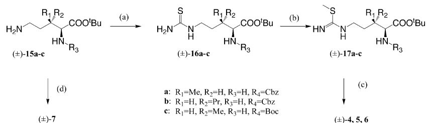
Scheme 3. Reagents and conditions: (a) (i) thiophosgene, CaCO_3 , CH_2Cl_2 , H_2O , rt, (ii) NH_3 , MeOH, 0^\circ C , 16a 77%, 16b 94%, 16c 54%; (b) MeI, CH_3CN , rt, 17a 80%, 17b 84%, 17c quant; (c) for 17a : HCl, THF, reflux; for 17b,c : (i) TFA, H_2O , phenol, thioanisole, 1,2-ethanedithiol, rt; for 17c : (ii) (–)ion exchange column, 4–6 quant; (d) (i) for 15a , ethyl acetimidate, K_2CO_3 , MeOH, rt, 23%, (ii) HCl, THF, reflux, quant.
