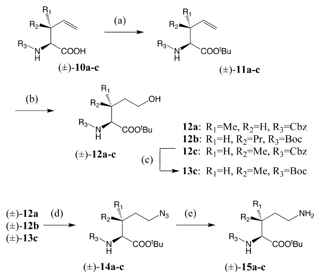
Scheme 2. Reagents and conditions: (a) isobutene, H 2 SO 4 , CH 2 Cl 2 , 0 °C, 11a 72%, 11b 31%, 11c 98%; (b) (i) hexylborane, THF, 0 °C, (ii) H 2 O 2 , pH 7.0, 12a 56%, 12b 78%, 12c 39%; (c) Pd/C, MeOH, (Boc) 2 O, Et 3 N, 13c 53%; (d) (i) MsCl, pyridine, CH 2 Cl 2 , 0 °C, (ii) NaN 3 , DMF, 50 °C, 14a 67%, 14b 42%, 14c 9.1%; (e) for 14a : Lindlar cat., MeOH, H 2 , rt; for 14b,c : Pd/C MeOH, H 2 , rt, 15a–c quant.
