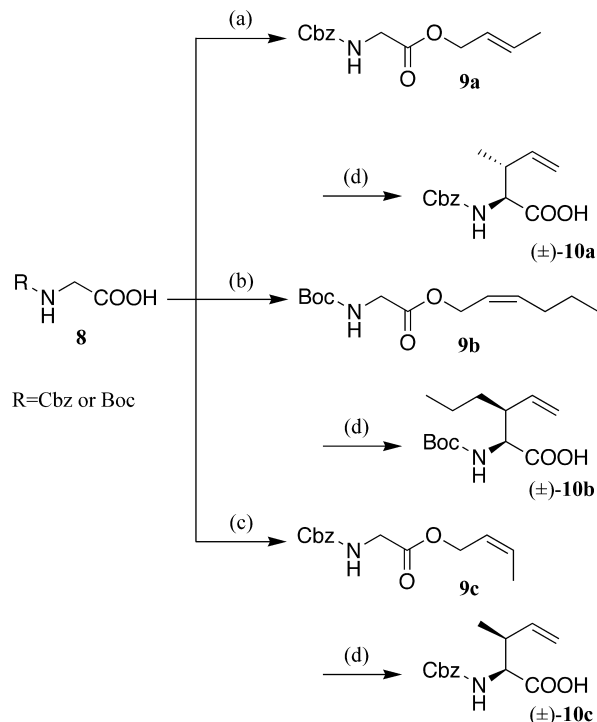
Scheme 1. Reagents and conditions: (a) crotyl alcohol, EDCI, DMAP, CH 2 Cl 2 , 0 °C, 95%; (b) cis -2-hexen-1-ol, EDCI, DMAP, CH 2 Cl 2 , 0 °C, 84%; (c) (i) 2-butyne-1-ol, EDCI, DMAP, CH 2 Cl 2 , 0 °C, (ii) Lindlar cat., MeOH, H 2 , rt, 99%; (d) LHMDS, Al( O - i -Pr) 3 , THF, −78 °C, 10a 52%, 10b 52%, 10c 30%.
