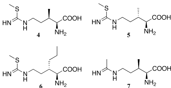
Figure 2. Design of 3-substituted arginine analogs.
